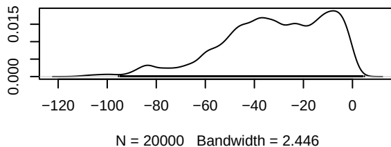
Density of d.II.II_HMGCRi
