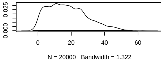
Density of d.I.I_PARPi
