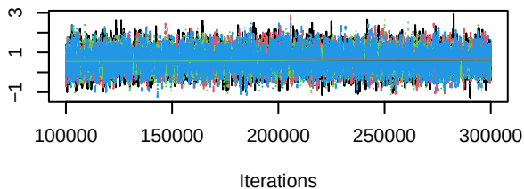
Trace of d.I.I_chemo
