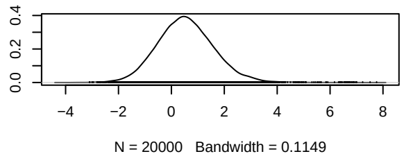
Density of d.I.Rociletinib
