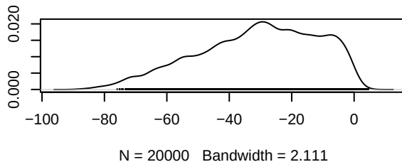
Density of d.I.I_COX2i
