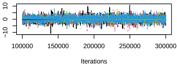
Trace of d.II.II_Cetuximab
